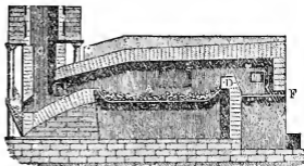
Fig. 3.—Puddling Furnace.
